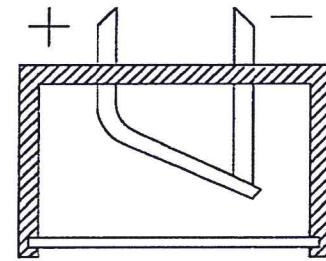
The diagram shows a detector for a fire alarm sprinkler system. When a fire raises the temperature, the positive (+) contact straightens and breaks the circuit, this will trigger the sprinklers.
